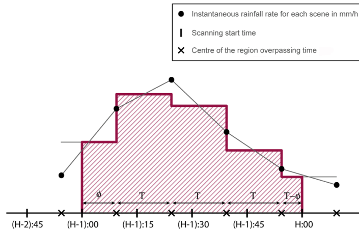
Figure 32. Trapezoidal integration
