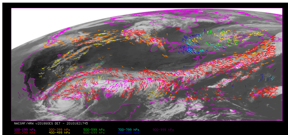
Figure 9: NWC/GEO-HRW v6.1 “Detailed AMV” output example in the Continental United States region (1 July 2010 17:45 UTC, GOES-13 satellite), considering default conditions defined in $SAFNWC/config/safnwc_HRW_GOESN.cfm model configuration file but with configurable parameter CDET = 1. Colour coding based on the AMV pressure level
