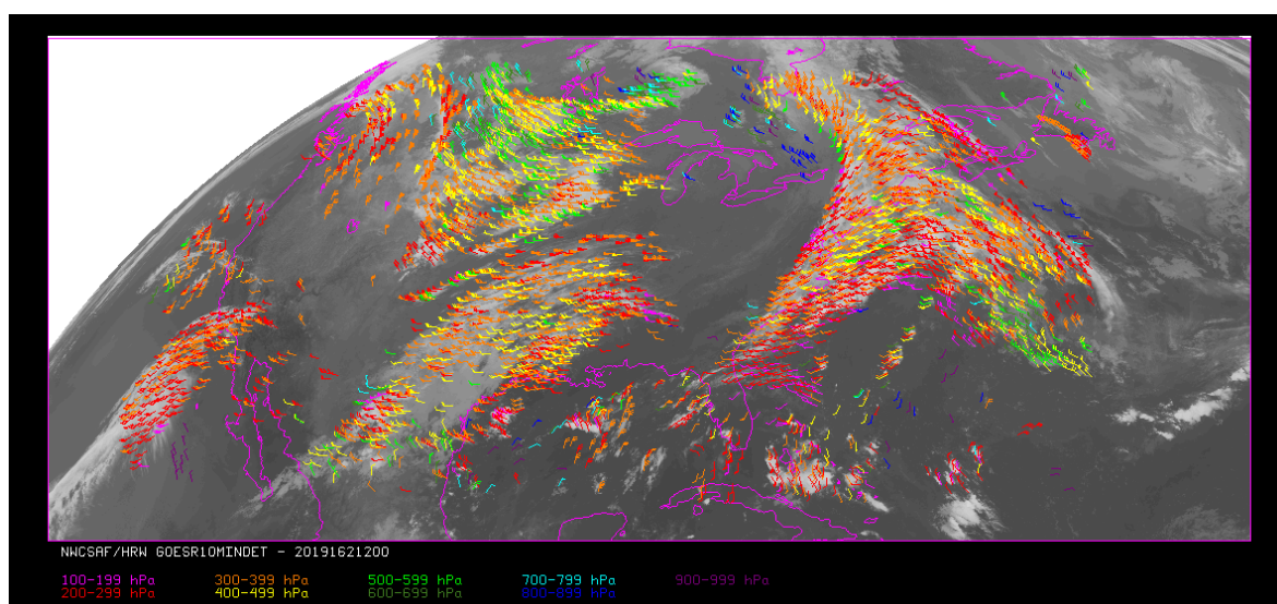
Figure 13: NWC/GEO-HRW v6.1 “Detailed AMV” output example in the Continental United States region (11 June 2019 12:00, GOES-16 satellite, “Mode 6”), considering the default conditions defined in $SAFNWC/config/safnwc_HRW_GOESR.cfm model configuration file. Colour coding based on the AMV pressure level
