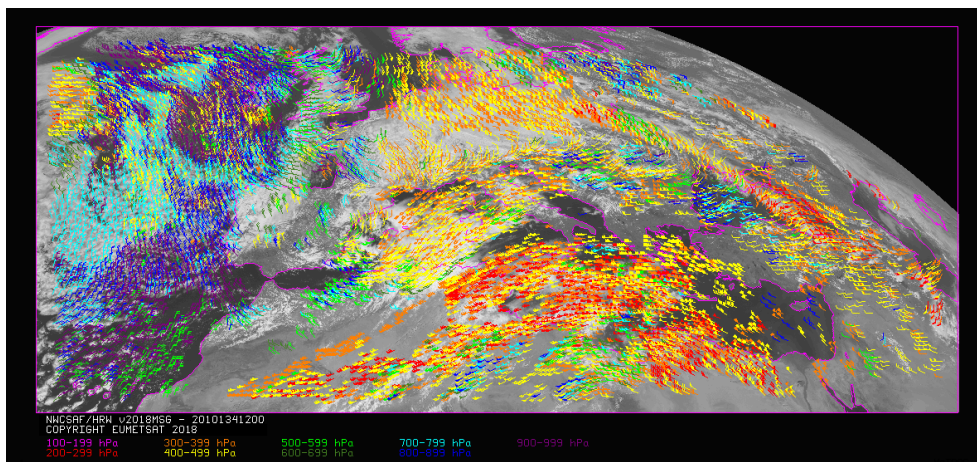
Figure 3: NWC/GEO-HRW v6.1 “Basic AMV” output example in the European and Mediterranean region (14 May 2010 12:00 UTC, MSG-2 satellite), considering default conditions defined in $SAFNWC/config/safnwc_HRW_MSG.cfm model configuration file but without Clouds products. Colour coding based on the AMV pressure level
