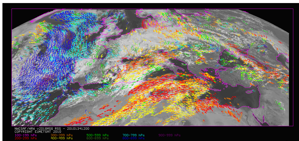
Figure 7: NWC/GEO-HRW v6.1 “Basic AMV” output example in the European and Mediterranean region (14 May 2010 12:00 UTC, MSG-1 satellite, Rapid scan mode), considering default conditions defined in $SAFNWC/config/safnwc_HRW_MSG.cfm model configuration file but with Mixed calculation method (with configurable parameters MIXED_SCANNING = 2 and SLOT_GAP = 2). Colour coding based on the AMV pressure level
