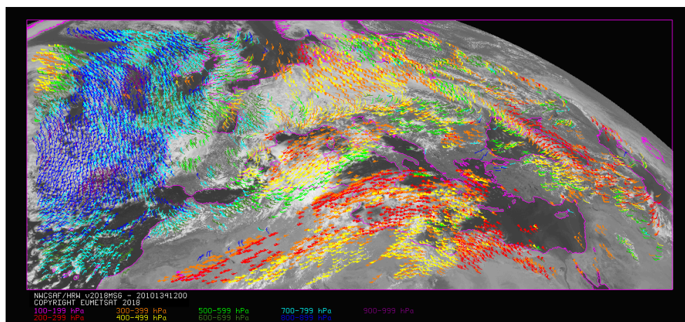
Figure 1: NWC/GEO-HRW v6.1 “Basic AMV” output example in the European and Mediterranean region (14 May 2010 12:00 UTC, MSG-2 satellite), considering default conditions defined in $SAFNWC/config/safnwc_HRW_MSG.cfm model configuration file. Colour coding based on the AMV pressure level
