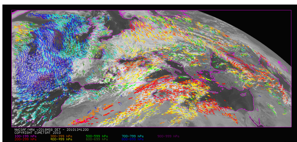
Figure 2: NWC/GEO-HRW v6.1 “Detailed AMV” output example in the European and Mediterranean region (14 May 2010 12:00 UTC, MSG-2 satellite), considering default conditions defined in $SAFNWC/config/safnwc_HRW_MSG.cfm model configuration file but with configurable parameter CDET = 1. Colour coding based on the AMV pressure level
