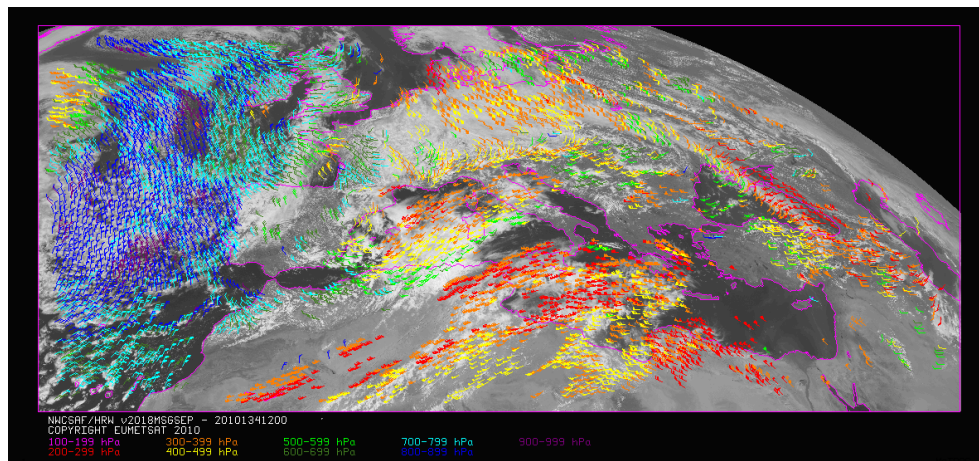
Figure 5: NWC/GEO-HRW v6.1 “Basic AMV” output example in the European and Mediterranean region (14 May 2010 12:00 UTC, MSG-2 satellite, Nominal scan mode), considering default conditions defined in $SAFNWC/config/safnwc_HRW_MSG.cfm model configuration file but with Mixed calculation method (with configurable parameters MIXED_SCANNING = 2 and SLOT_GAP = 2). Colour coding based on the AMV pressure level
