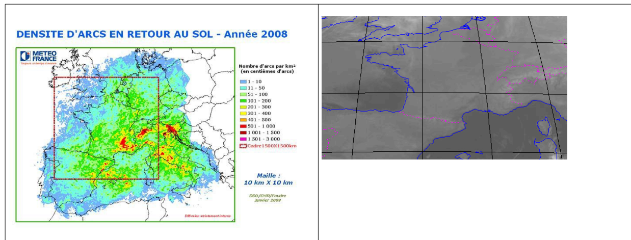
Figure 21: Left: Extension and quality (density) of Meteorage+partners network. Meteorage network coverage appears in red. Left: Domain used for GEN discrimination tuning
