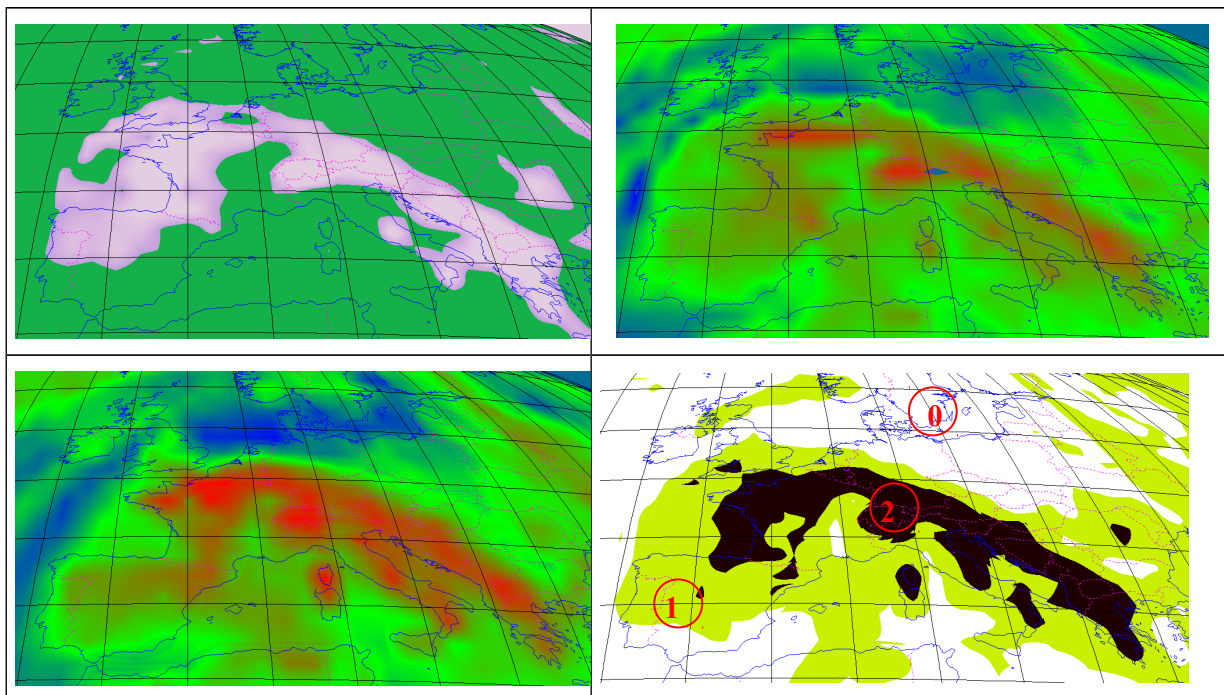
Figure 1: 25 May 2009, 12h15. Convective mask (bottom right), as a union of K index (top left), Showalter index (top right) and Lifted index (bottom left), from NWP data. Regions 1 and 2 are region of interest for analysis
