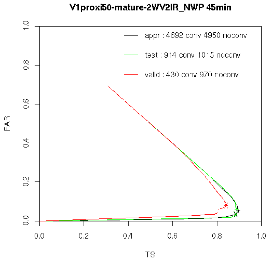
Figure 23: MSG v2011 tuning. TS/FAR curves for mature discrimination (DM), full configuration 6.2 \mu m+7.3 \mu m +8.7 \mu m +10.8 \mu m +12.0 \mu m +NWP, 45 min depth, for a moderate ground truth with proximity to flashes taken into account Learning database (black), random test database (green), Validation database(red)
