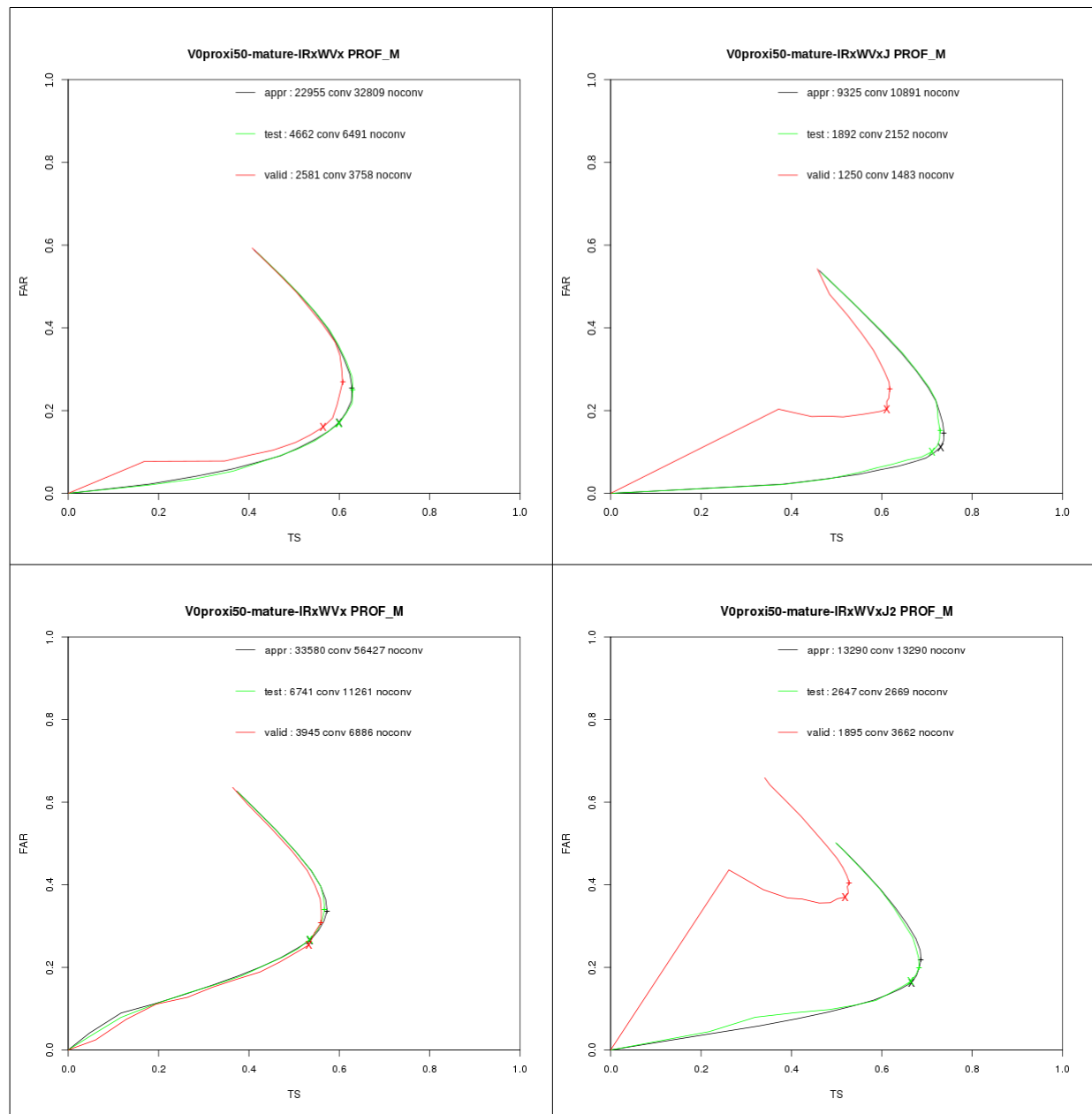
Figure 24: MSG4 (top) and Himawari8 (bottom) tuning results for mature discrimination (DM), nominal (left) and day-time (right) configurations, for medium depths (30min MSG, 40min
