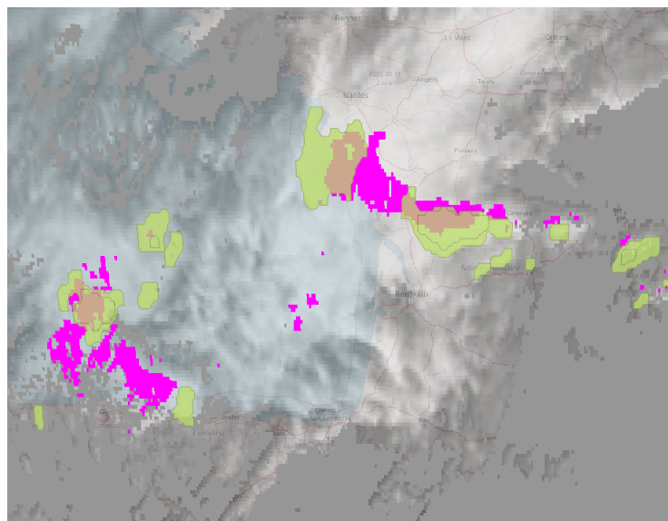
Figure 26: 13th june 2017, 15h00Z, Biscay bay. Illustration of 2D field of icing index derived from CMIC parameters (magenta), superimposed with RDT cells (green). Cells including highlighted pixels are associated with high altitude icing hazard attribute set to 1
