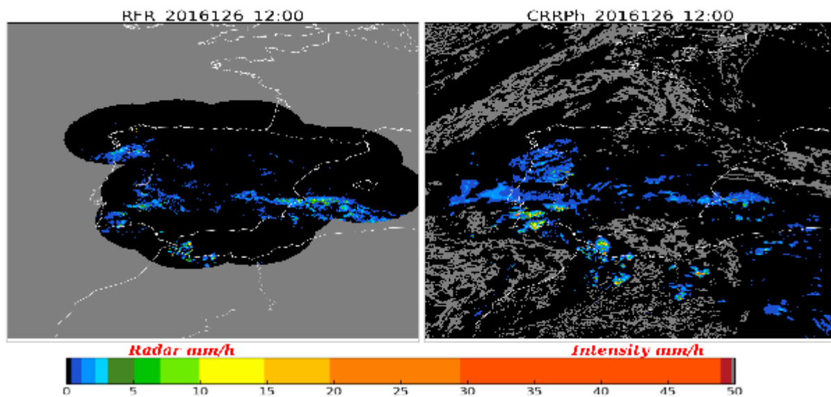
Figure 36. Comparison of radar (PPI) and CRR-Ph day product on 5 th May 2016 at 12:00UTC
