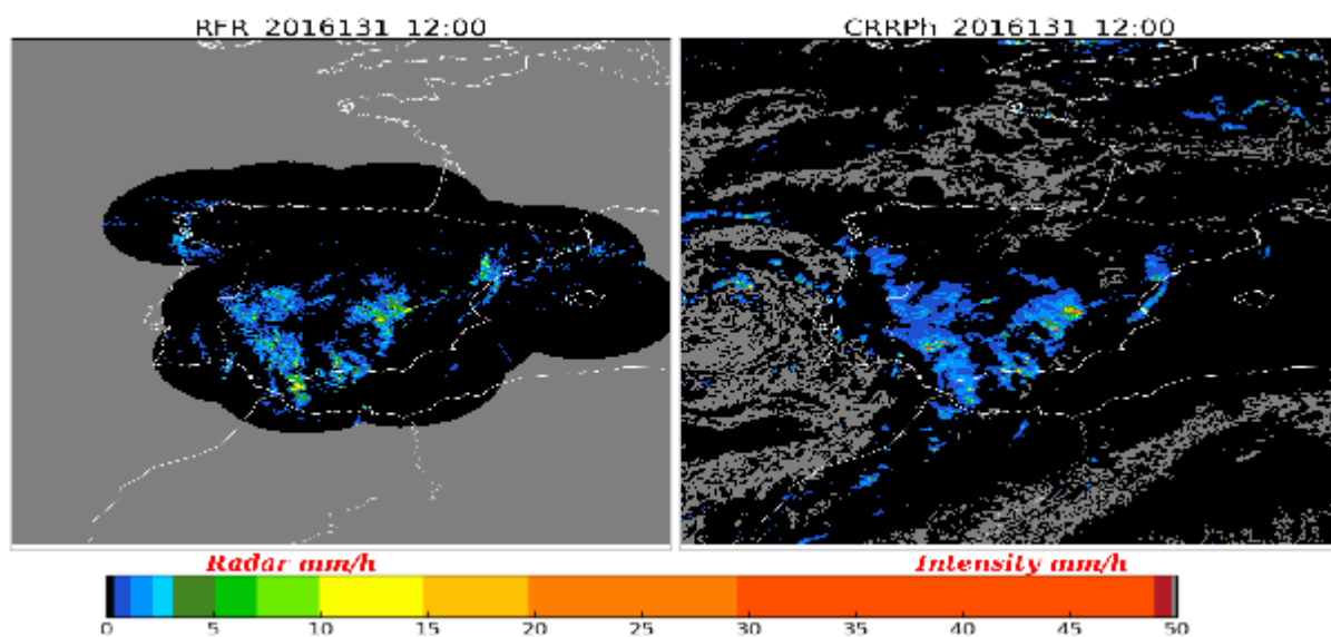
Figure 41. Comparison of radar (PPI) and CRR-Ph day product on 10 th May 2016 at 12:00UTC
