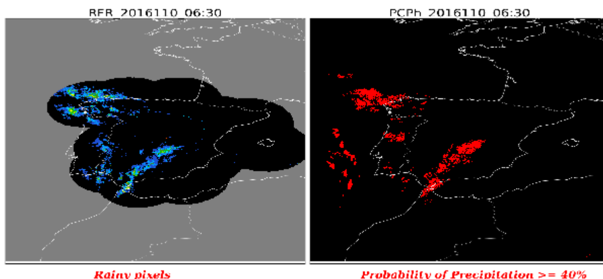
Figure 33. Comparison of radar (PPI) and probability of precipitation equal or higher to 40% extracted from PC-Ph product on 19 th April 2016 at 6:30UTC
