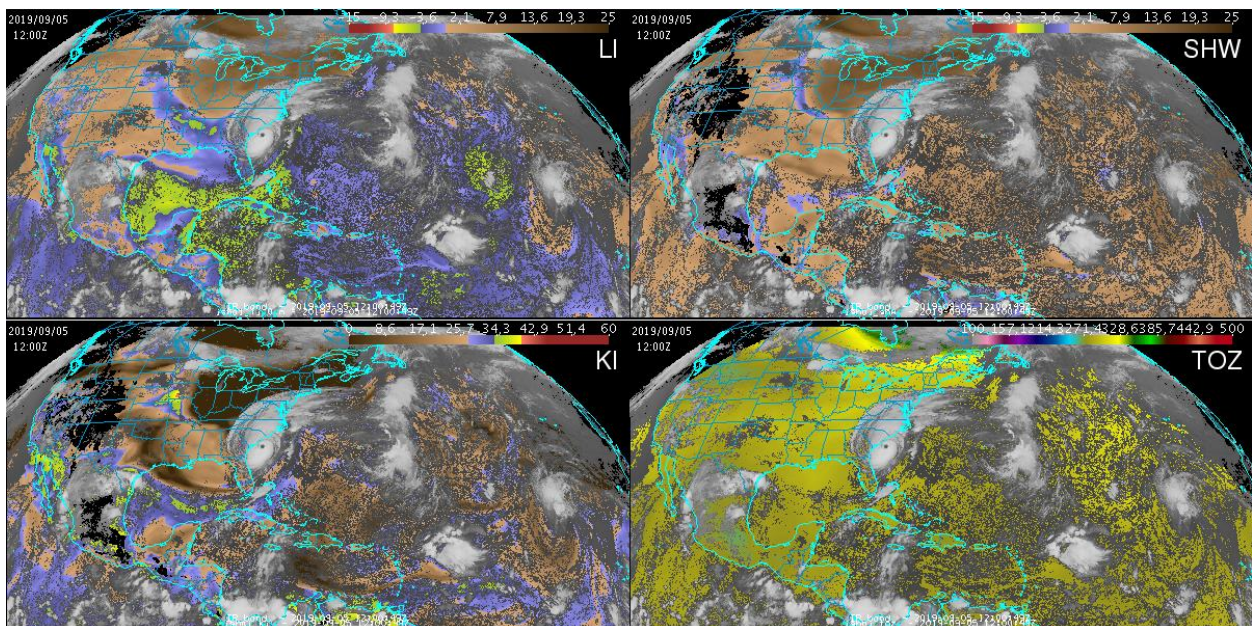
Figure 18: Example of GEO-iSHAI LI, SHW, KI and TOZ from 12 UTC on 5 September 2019 produced from ABI on GOES-16.
