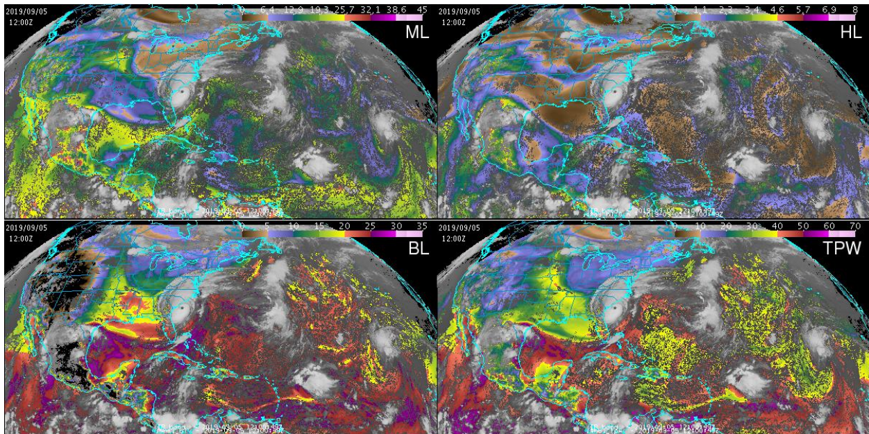
Figure 17: Example of GEO-iSHAI BL, ML, HL and TPW from 12 UTC on 5 September 2019 produced from ABI on GOES-16.
