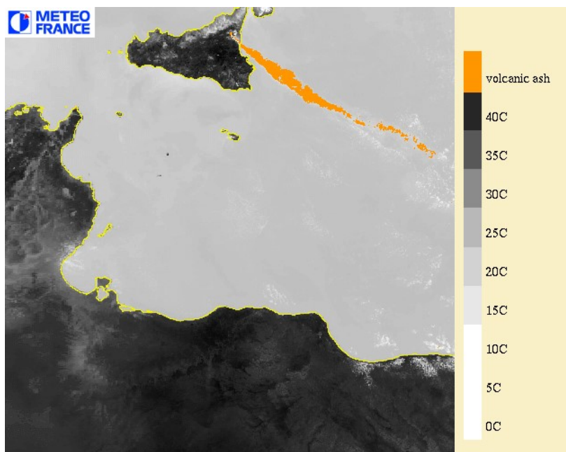
Figure 2: Example of MODIS volcanic ash cloud superimposed on a 10.8μm infrared image: Etna eruption on 22th July 2001 at 9h55 UTC.
