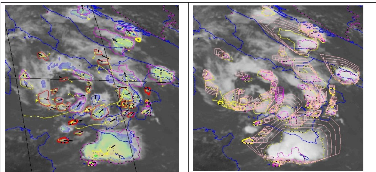
Figure 25: 11 th August 2015 09h00 UTC slot – illustration of RDT advection scheme. Left: analysed RDT-CW cells with motion vectors. Right: RDT-CW +15, +30, +45 and +60 smoothed and dilated forecast cells
