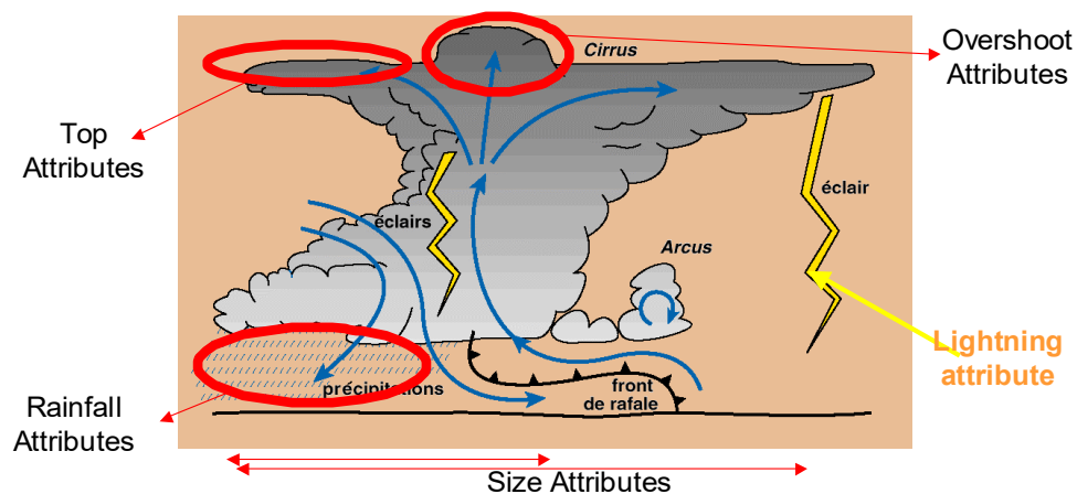
Figure 9: RDT-CW scheme
