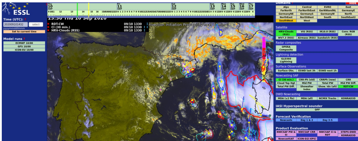
Figure 10: ESSL visualization
