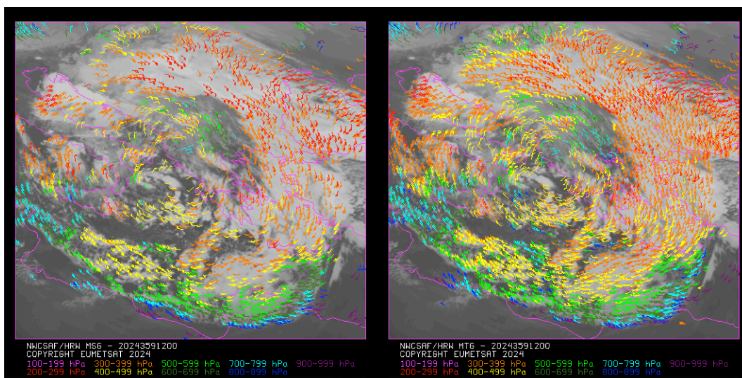
Figure 5: Comparison of NWC/GEO-High Resolution Winds v7.0.1 Basic AMV output for 24 December 2024 12:00 UTC for Meteosat-10 satellite (left) and Meteosat-12 (MTG-I1) satellite (right) around a low pressure area over the Ionian Sea
