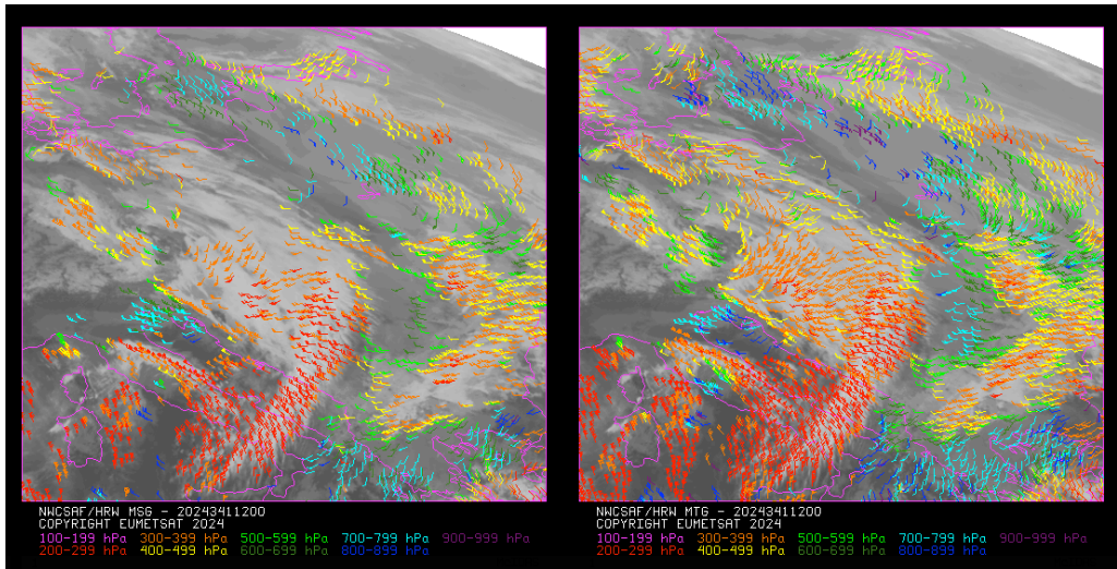
Figure 6: Comparison of NWC/GEO-High Resolution Winds v7.0.1 Basic AMV output for 6 December 2024 12:00 UTC for Meteosat-10 satellite (left) and Meteosat-12 (MTG-I1) satellite (right) in the Eastern European region
