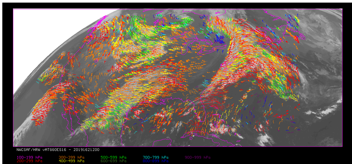
Figure 11: NWC/GEO-High Resolution Winds v7.0.1 Basic AMV output example in the Continental United States region (11 June 2019 12:00 UTC, GOES-16 satellite), considering default conditions in $SAFNWC/config/GOES*/safnwc_HRW.cfm model configuration file. Colour coding based on the AMV pressure level
