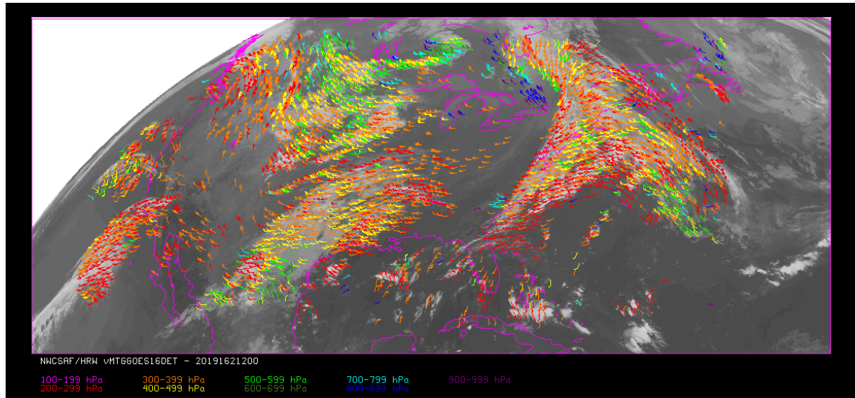
Figure 12: NWC/GEO-High Resolution Winds v7.0.1 Detailed AMV output example in the Continental United States region (11 June 2019 12:00 UTC, GOES-16 satellite), considering default conditions in $SAFNWC/config/GOES*/safnwc_HRW.cfm model configuration file and configurable parameter CDET = 1. Colour coding based on the AMV pressure level
