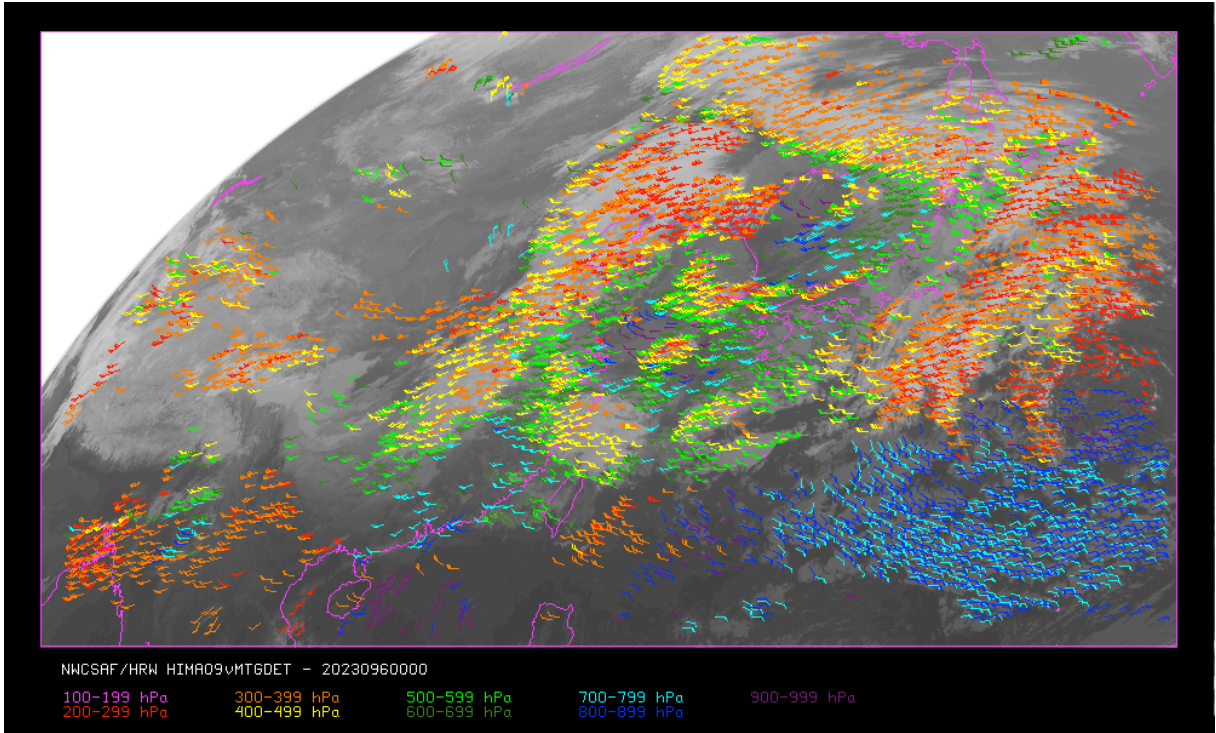
Figure 10: NWC/GEO-High Resolution Winds v7.0.1 Detailed AMV output example in the China/Korea/Japan region (6 April 2023 00:00 UTC, Himawari-9 satellite), considering default conditions in $SAFNWC/config/HIMA*/safnwc_HRW.cfm model configuration file and configurable parameter CDET = 1. Colour coding based on the AMV pressure level
