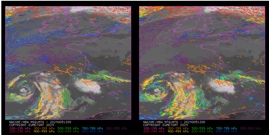
Figure 7: Comparison of NWC/GEO-High Resolution Winds v7.0.1 Basic AMV output for 31 October 2024 12:00 UTC for Meteosat-10 satellite (left) and Meteosat-12 (MTG-I1) satellite (right) in the region around the Bay of Biscay
