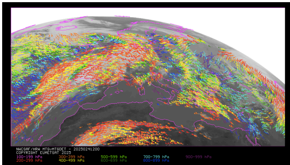
Figure 4: NWC/GEO-High Resolution Winds v7.0.1 Detailed AMV output example in the European and Mediterranean region (24 January 2025 12:00 UTC, Meteosat-12 (MTG-I1) satellite data), considering default conditions in $SAFNWC/config/MTI*/safnwc_HRW.cfm model configuration file and configurable parameter CDET = 1. Colour coding based on the AMV pressure level
