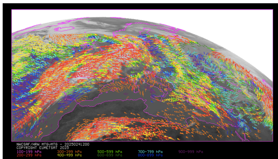
Figure 3: NWC/GEO-High Resolution Winds v7.0.1 Basic AMV output example in the European and Mediterranean region (24 January 2025 12:00 UTC, Meteosat-12 (MTG-I1) satellite data), considering default conditions in §SAFNWC/config/MTI1*/safnwc_HRW.cfm model configuration file. Colour coding based on the AMV pressure level
