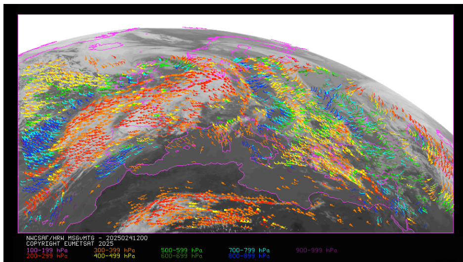
Figure 1: NWC/GEO-High Resolution Winds v7.0.1 Basic AMV output example in the European and Mediterranean region (24 January 2025 12:00 UTC, Meteosat-10 satellite), considering default conditions in SAFNWC/config/MSG*/safnwc_HRW.cfm model configuration file. Colour coding based on the AMV pressure level
