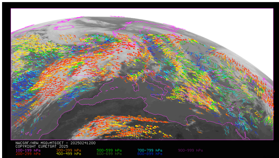
Figure 2: NWC/GEO-High Resolution Winds v7.0.1 Detailed AMV output example in the European and Mediterranean region (24 January 2025 12:00 UTC, Meteosat-10 satellite), considering default conditions in $SAFNWC/config/MSG*/safnwc_HRW.cfm model configuration file and configurable parameter CDET = 1. Colour coding based on the AMV pressure level
