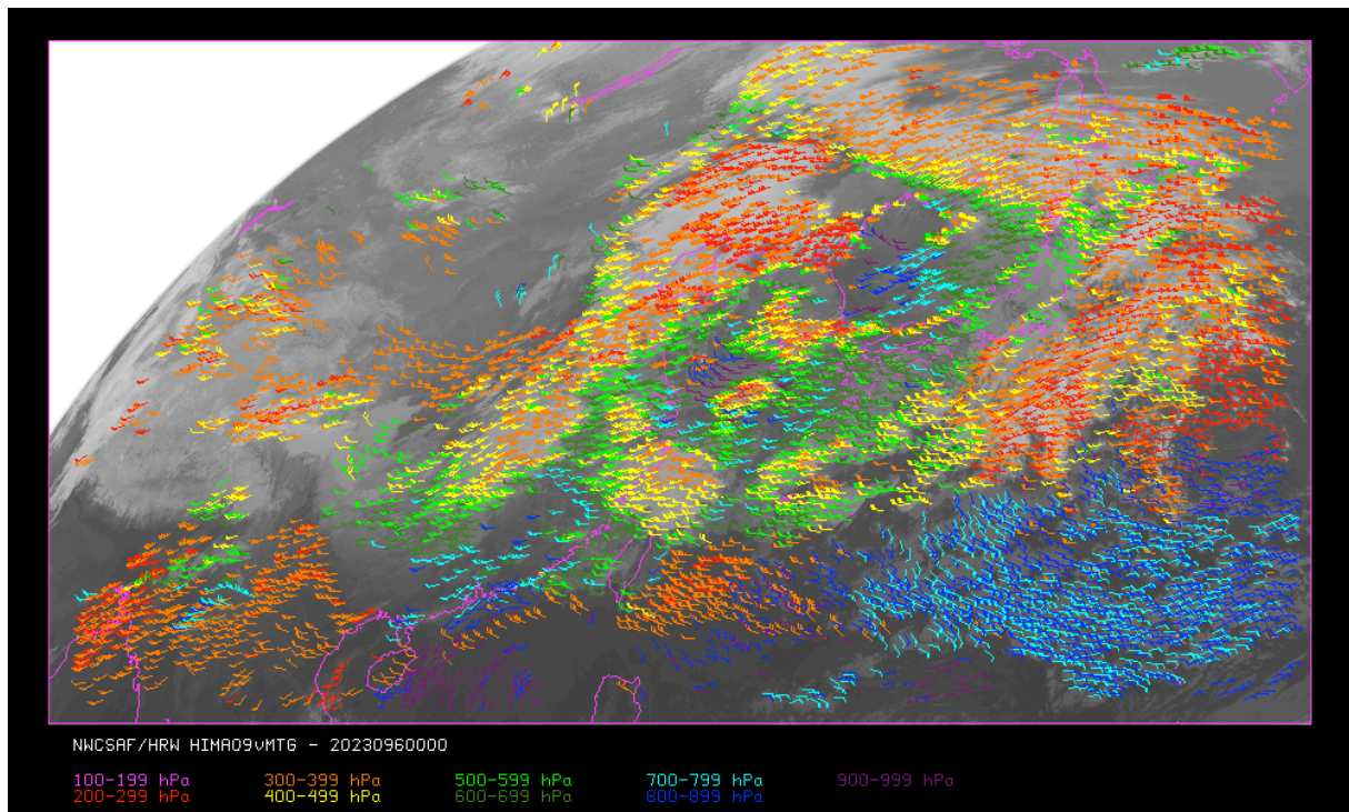
Figure 9: NWC/GEO-High Resolution Winds v7.0.1 Basic AMV output example in the China/Korea/Japan region (6 April 2023 00:00 UTC, Himawari-9 satellite), considering default conditions in $SAFNWC/config/HIMA*/safnwc_HRW.cfm model configuration file. Colour coding based on the AMV pressure level
