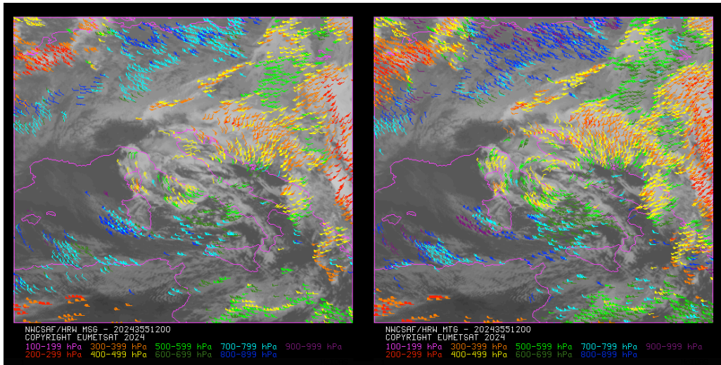
Figure 8: Comparison of NWC/GEO-High Resolution Winds v7.0.1 Basic AMV output for 20 December 2024 12:00 UTC for Meteosat-10 satellite (left) and Meteosat-12 (MTG-I1) satellite (right) in Central Europe and Italy
