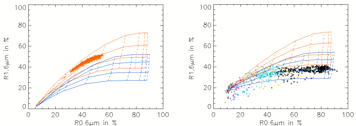
Figure 44 Illustration of the cloud phase retrieval using 0.6μm and 1.6μm reflectances. Cloud measurements (coloured using CT cloud type colors, except white color replaced by black) are superimposed to simulated curves. Left: for a maritime stratocumulus cloud; right: for a convective system over the Pyrenees.
