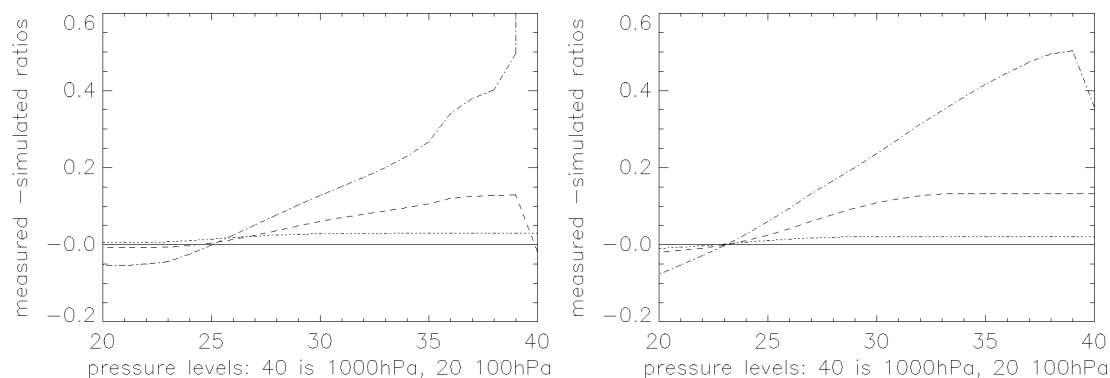
Figure 38: Illustration of the Radiance Ratioing technique applied to SEVIRI radiances.
