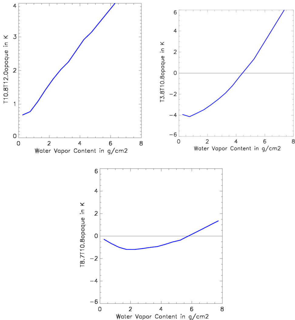
Figure 33: Illustration of T108T120opaque, T38T108opaque and T87T108opaque for a satellite zenith angle of 48 degrees
