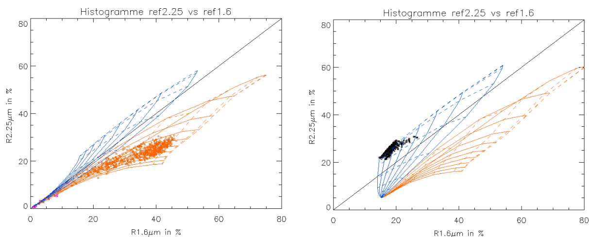
Figure 43 Illustration of the cloud phase retrieval using 1.6 \mu m and 2.25 \mu m reflectances from Himawari. Cloud measurements (coloured using CT cloud type colors, except white color replaced by black) are superimposed to simulated curves. Left: for a maritime stratus cloud; right: for a convective system.
