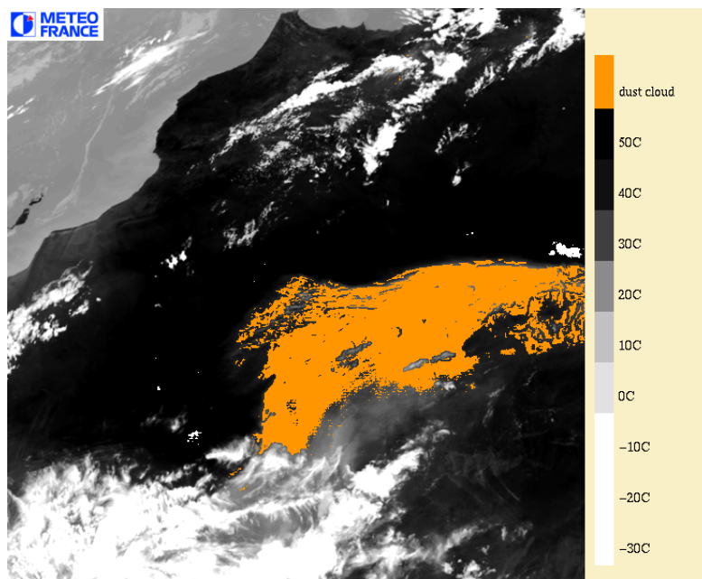
Figure 31: Example of SEVIRI dust cloud flag superimposed on a 10.8 \mu m infrared image: dust cloud over North Africa on 14 th July 2003 at 13h00 UTC.
