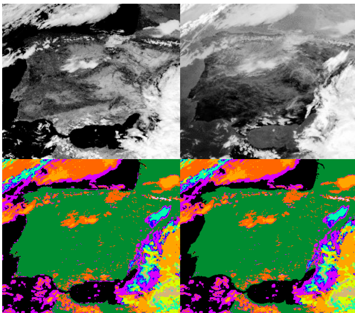
Figure 28 Illustration of spatial filtering effect in coastal area, 28 November 2007 12h00UTC top left VIS 0.6, top right IR T10.8; bottom left, CT without coastal filtering; bottom right CT with coastal filtering
