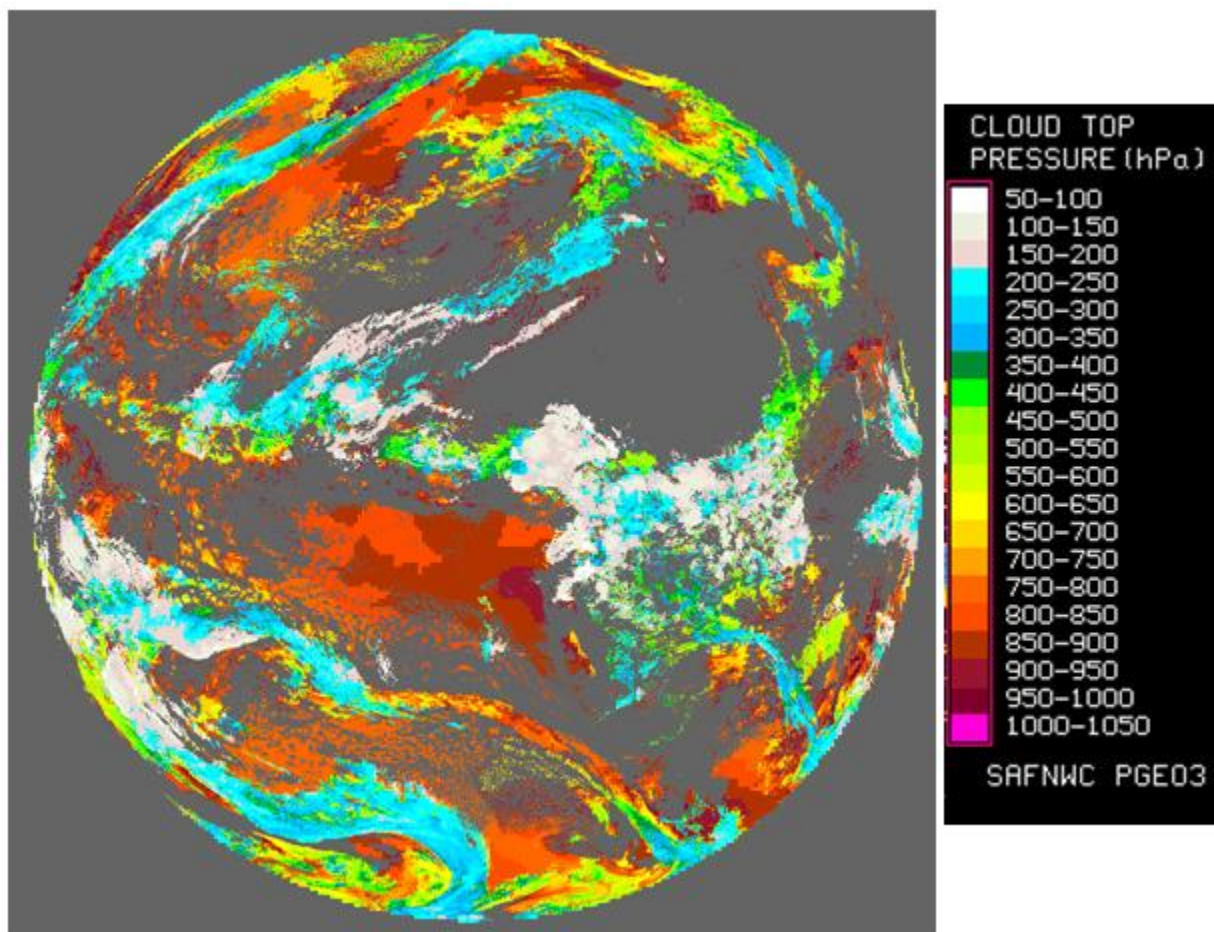
Figure 41: Example of SEVIRI CTTH cloud top pressure
