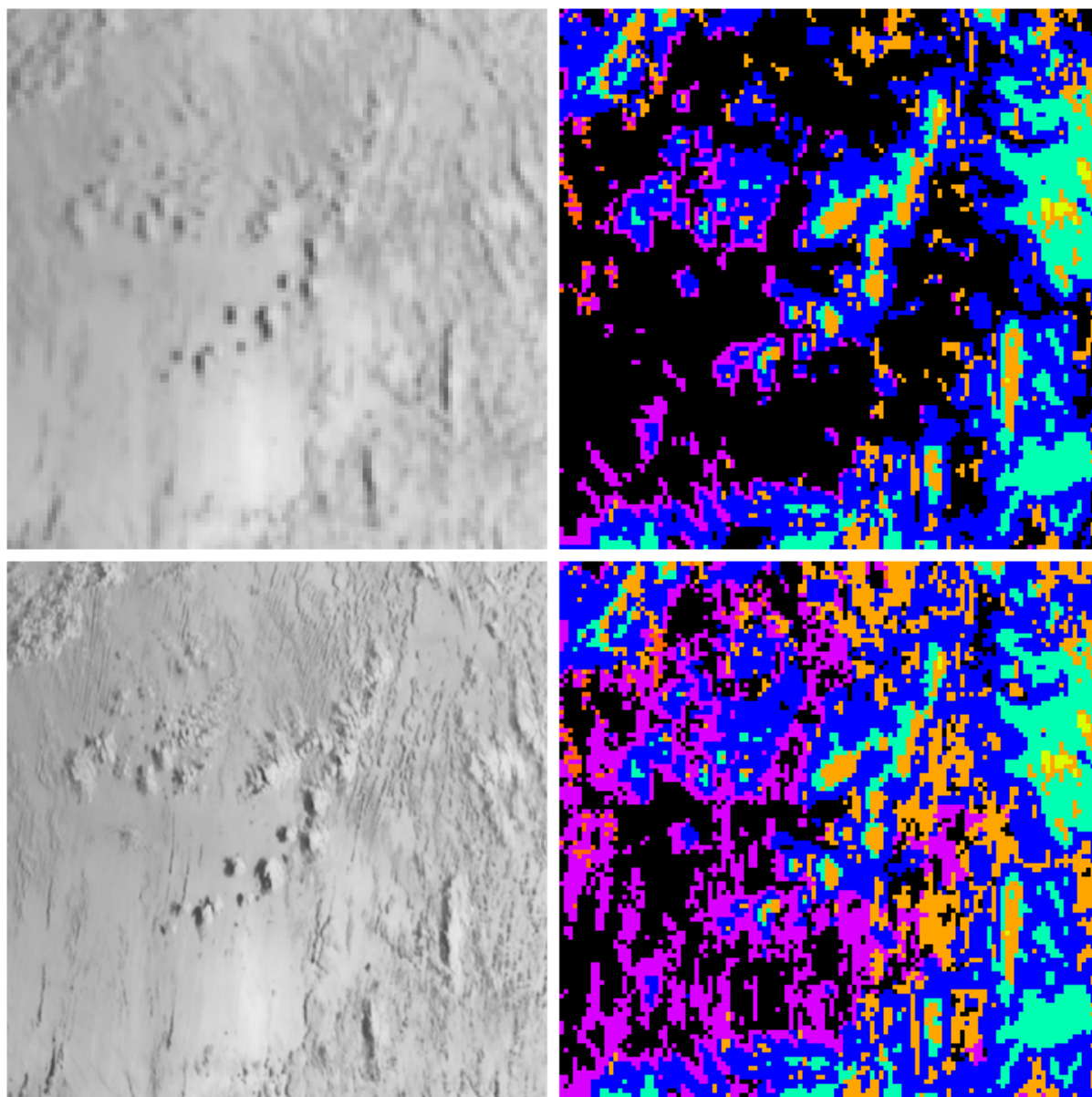
Figure 23 Sunlint with trade-wind convective low clouds over Indian Ocean, 8 September 2009, 04h00UTC, (120x120 at low resolution SEVIRI scale). Top left: 0.8 \mu\text{m} visible reflectance; top right: v2009 cloud type; bottom left: HRV reflectance; bottom right: v2010 cloud type
