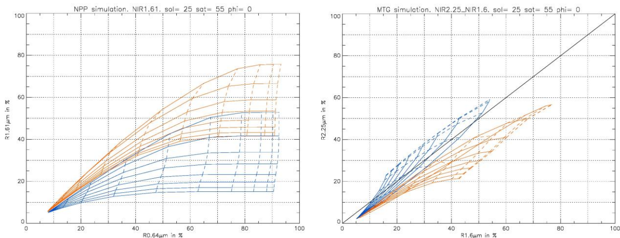
Figure 42 Illustration of the simulation of 0.6\mu m/1.6\mu m and 1.6\mu m/2.25\mu m cloud reflectances for a selection of water (in orange) and ice (in blue) cloud models for a given oceanic location (fixed viewing angles and surface cloud-free reflectances).
