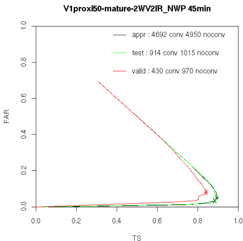
Figure 23: MSG v2011 tuning. TS/FAR curves for mature discrimination, full configuration 6.2\mu\text{m}+7.3\mu\text{m}+8.7\mu\text{m}+10.8\mu\text{m}+12.0\mu\text{m}+\text{NWP} , 45-min depth, for a moderate ground truth with proximity to flashes taken into account. Learning database (black), random test database (green), validation database (red)
