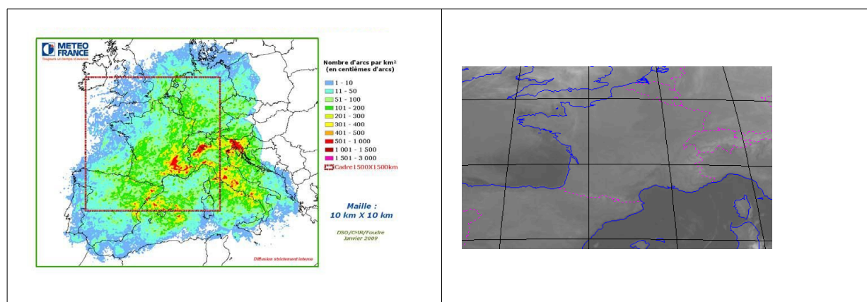
Figure 21: Left: Extension and quality (density) of Meteorage+partners network. Meteorage network coverage appears in red. Right: Domain used for GEN discrimination tuning
