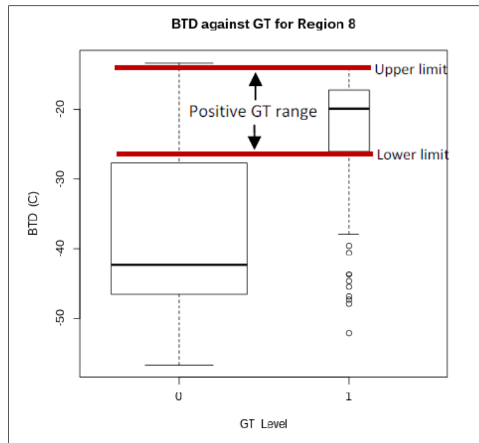
Figure 8: Analysis of an interest field parameter (here BTD) from pre-CI pixels on a selected region vs Radar Ground Truth. Ranges of values are assessed or tuned through this approach.
