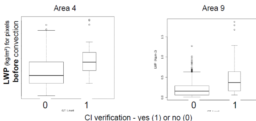
Figure 3: Box-plots for two regions and test cases used to define threshold for LWP. From [R.D. 2]
