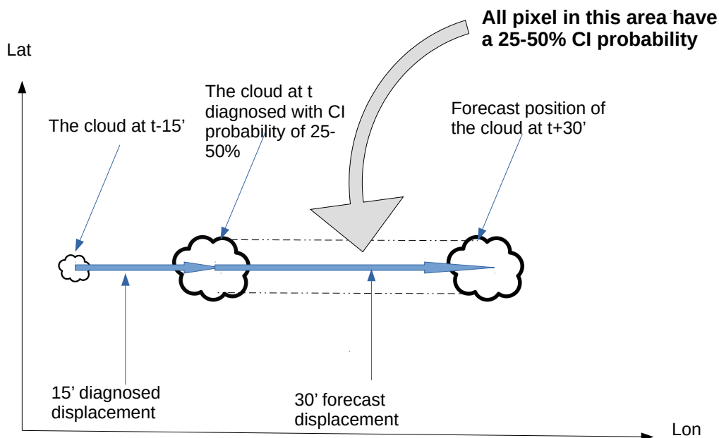
Figure 4: Forward scheme of CI. The CI diagnosis can only be extrapolated to CI-eligible pixels. In the event of several CI signals competing for the same pixel, the highest probability is kept.
