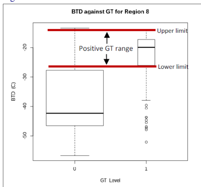
Figure 8: Analysis of an interest field parameter (here BTD) from pre eligible-CI pixels on a selected region vs Radar Ground Truth. Ranges of values are assessed or tuned through this approach.
