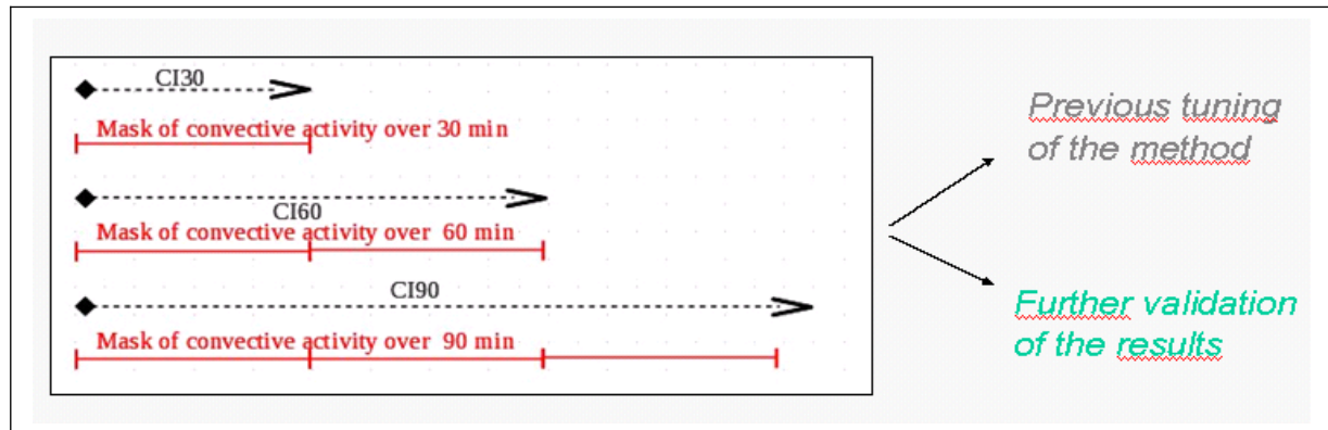
Figure 6: preEligible-CI pixels vs different Ground Truth masks
