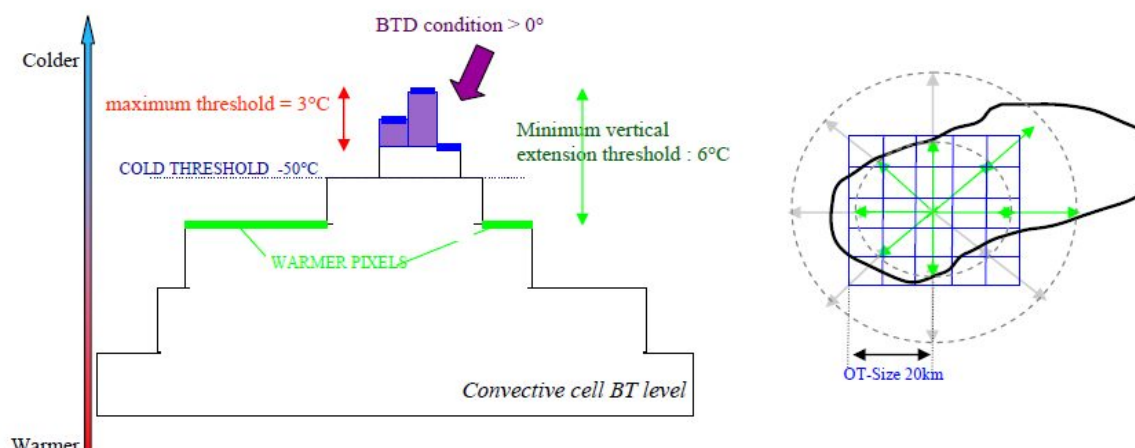
Figure 27: First step of OT detection: Values of criteria for vertical morphological analysis (left), illustration of a horizontal analysis (right). Arrows point surrounding pixels to check (green when belonging to the cloud cell), blue grid represent the research window for OT extension.
