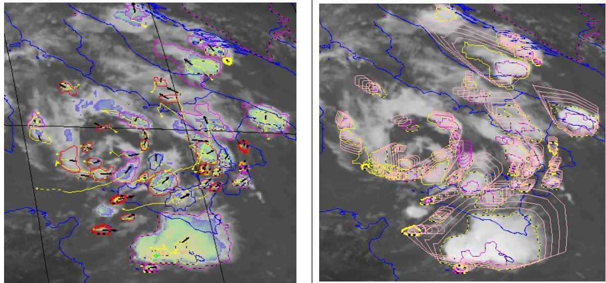
Figure 25: 11 th August 2015 09h00 UTC slot – illustration of RDT advection scheme. Left: analysed RDT-CW cells with motion vectors. Right: RDT-CW +15, +30, +45 and +60 smoothed and dilated forecast cells
