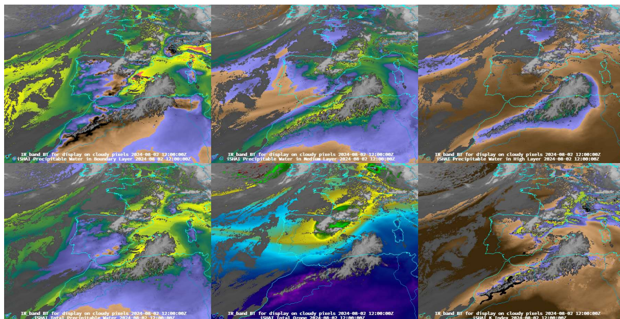
Figure 4: Example of GEO-iSHAI BL, ML, HL, TPW, TOZ and KI from 12 UTC on 2 August 2024 produced from FCI on MTG-II.
