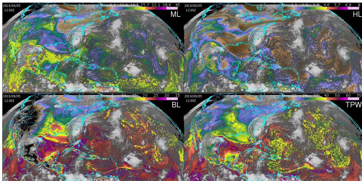
Figure 13: Example of GEO-iSHAI BL, ML, HL and TPW from 12 UTC on 5 September 2019 produced from ABI on GOES-16.
