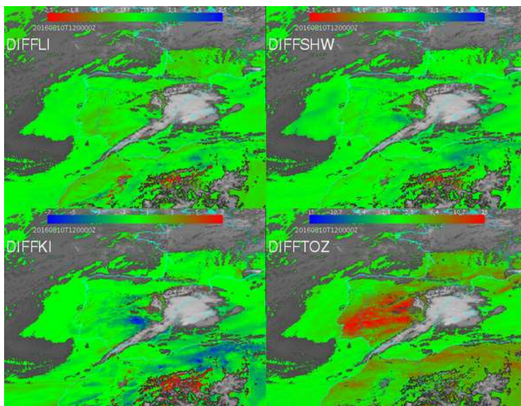
Figure 8: Example of GEO-iSHAI diffLI, diffSHW, diffKI and diffTOZ from 12 UTC on 10 August 2016 produced from MSG-3.
