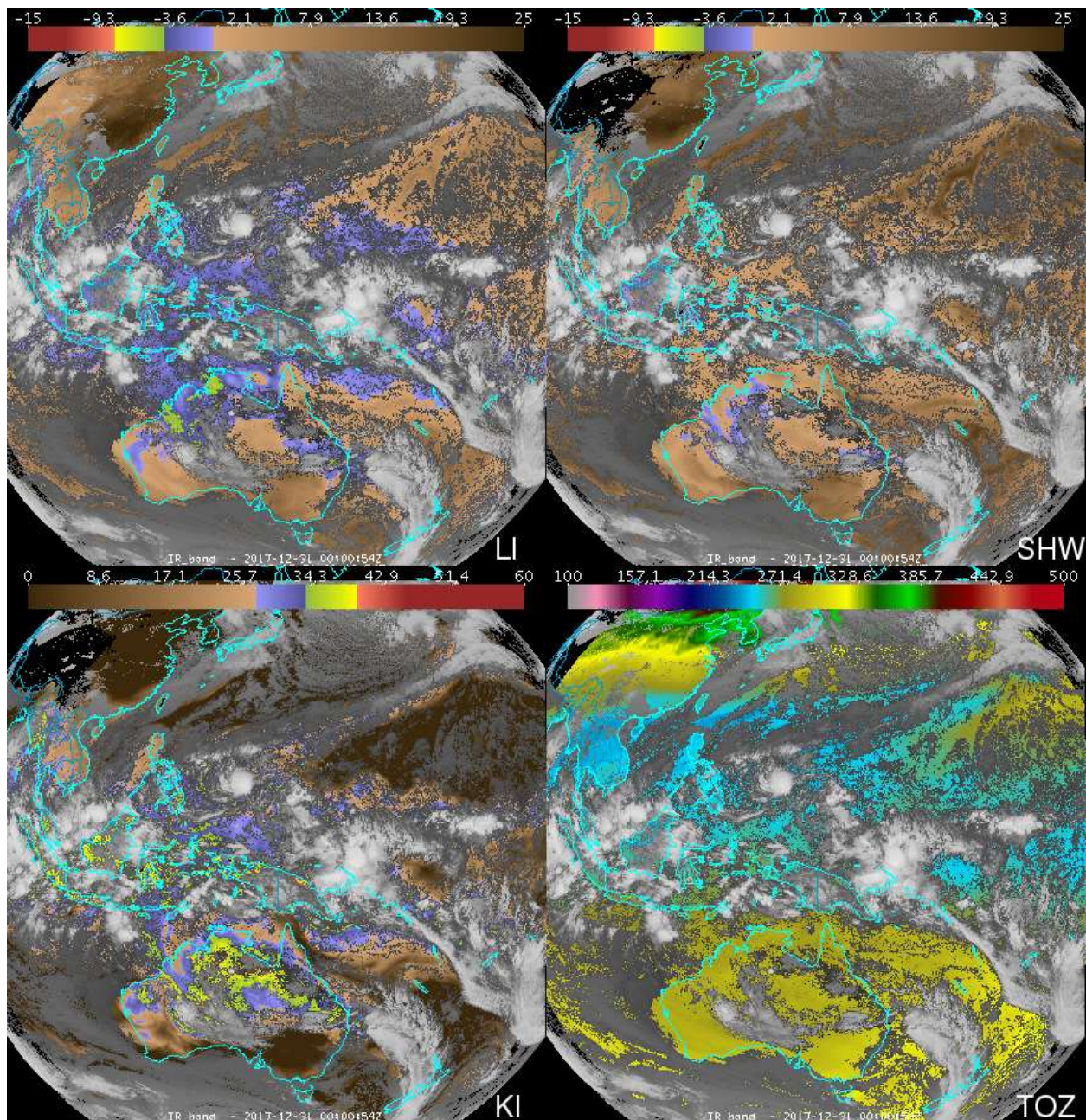
Figure 12: Example of GEO-iSHAI LI, SHW, KI and TOZ from 12 UTC 31 December 2017 produced from AHI on Himawari-8.
