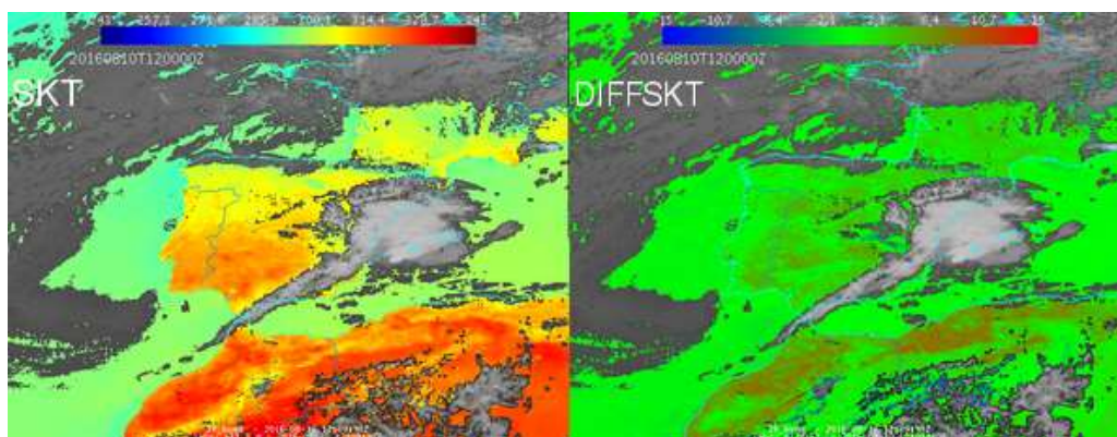
Figure 9: Example of GEO-iSHAI SKT and diffSKT 12 UTC on 10 August 2016 produced from MSG-3.
