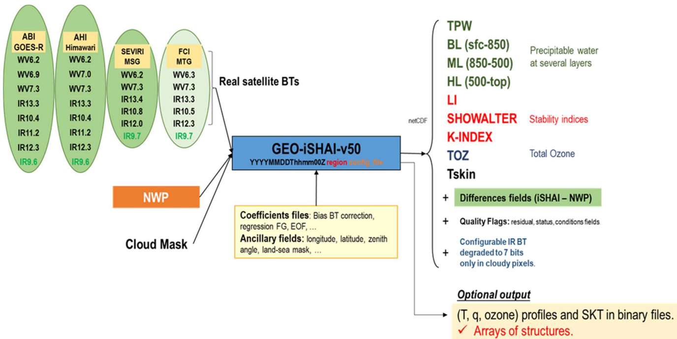
Figure 1: GEO-iSHAI inputs and outputs scheme
