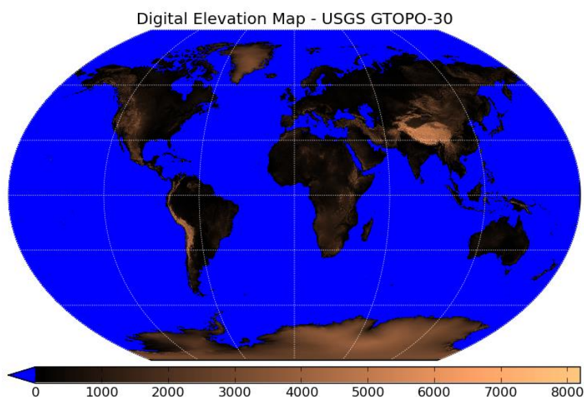
Figure 2: The digital elevation map used in PPS
