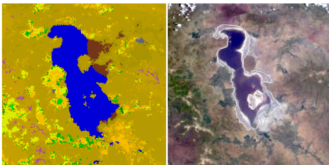
Figure 5: Usgs Landuse map (left) and S-NPP VIIRS True Color image taken June 5 th , 2013, 10:41 UTC received and processed at SMHI. The area in focus is the Lake Urmia in Northeastern Iran.
