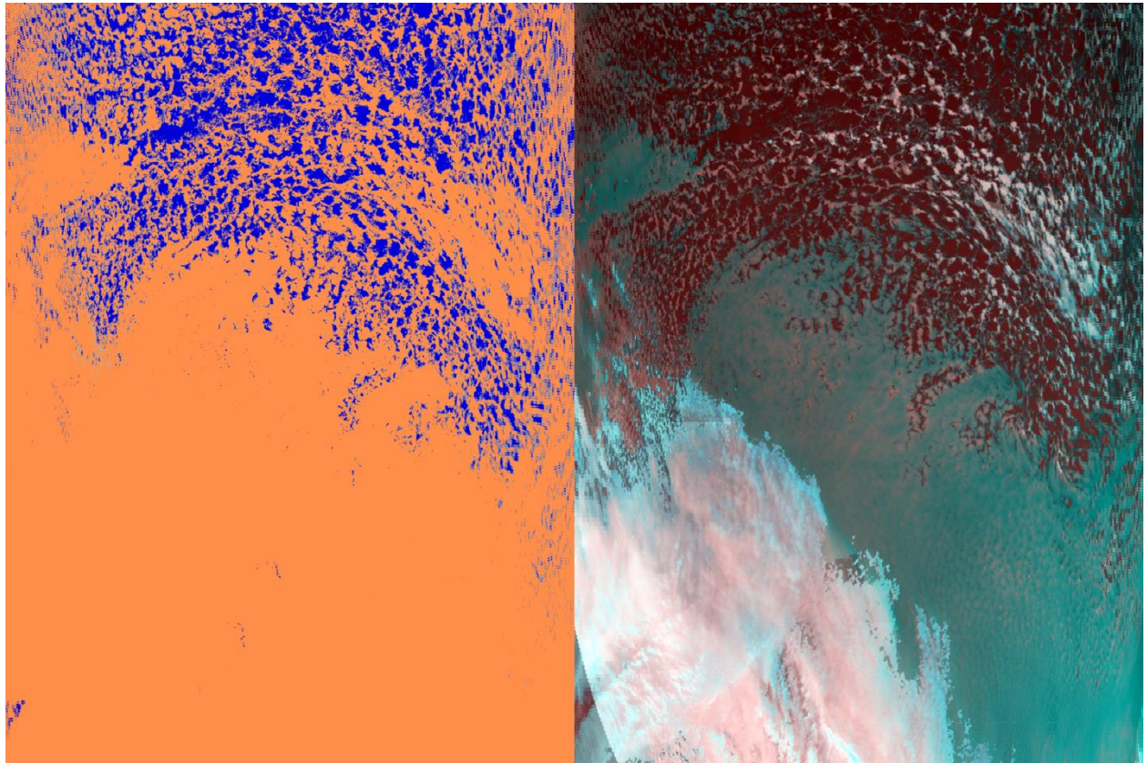
Figure 1 Showing PPS CMa applied to simulated EPS-SG-A data (2007-09-12 09:08UTC). Note that data are simulated.
