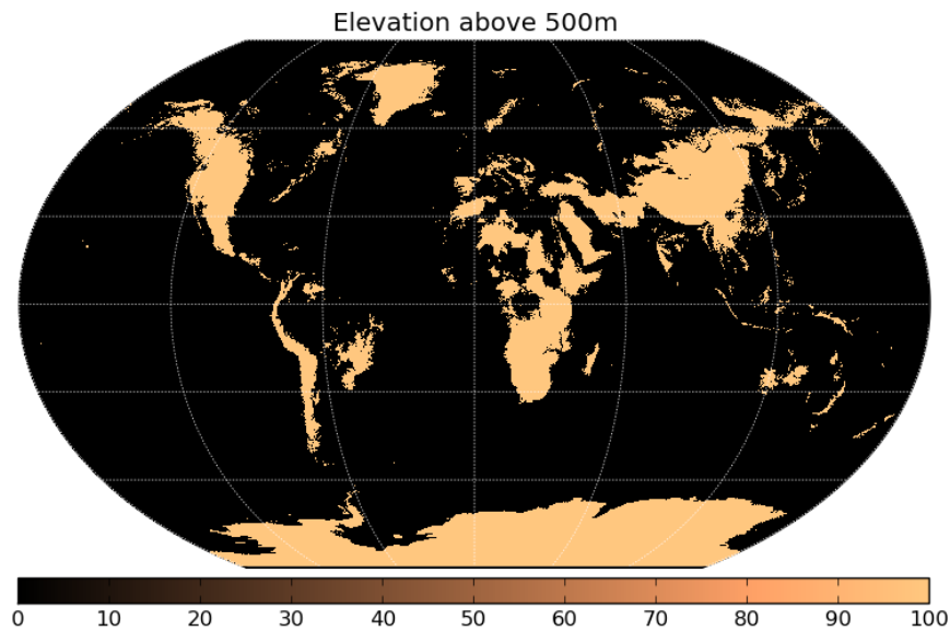
Figure 3: Global map highlighting areas on the earth with an elevation above 500 meters. The 500 meter limit was used previously in PPS to delineate low-land from mountainous terrain.
