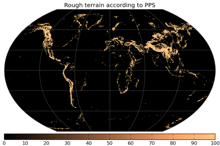
Figure 4 Global map showing where on earth the terrain is rough according to PPS. This is the dataset used in PPS from version 2014 to delineate rough/mountainous terrain from low-land/gentle terrain.
