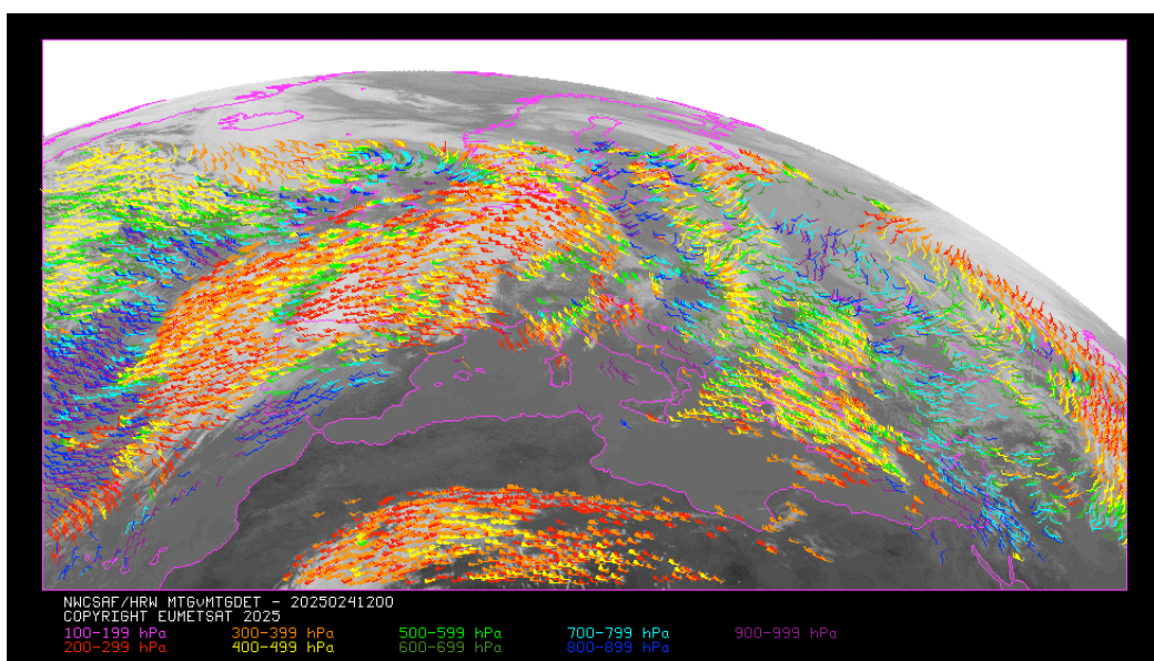
Figure 33: NWC/GEO-High Resolution Winds v7.0 Detailed AMV output example in the European and Mediterranean region (24 January 2025 12:00 UTC, Meteosat-12 (MTG-I1) satellite), considering default conditions in $SAFNWC/config/MTI*/safnwc_HRW.cfm model configuration file. Colour coding based on the AMV pressure level
