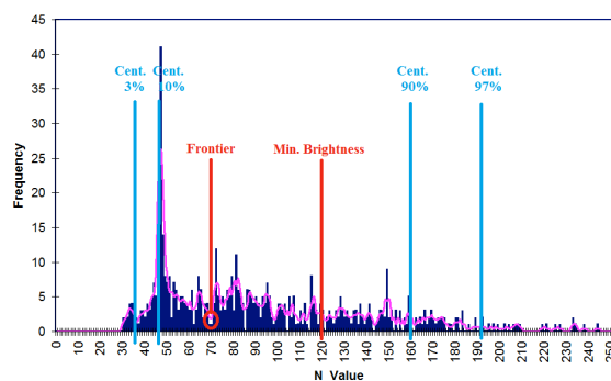
Figure 1: Example of “N_Value matrix histogram” (unsmoothed in violet and smoothed in pink) for a valid low resolution “tracer candidate”. The minimum brightness threshold, the algorithm centiles and the defined frontier are also shown
