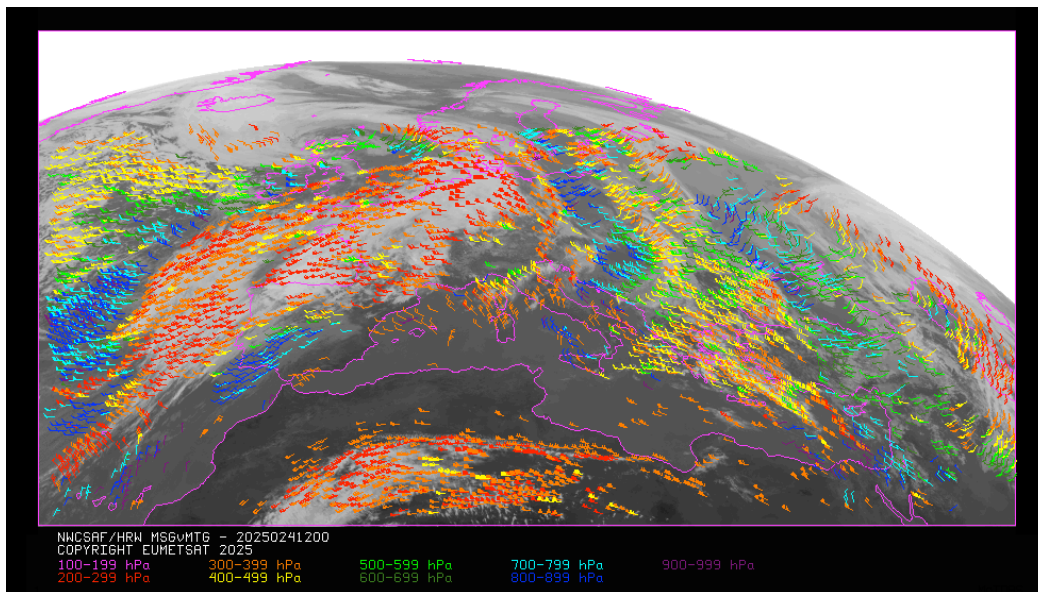
Figure 34: NWC/GEO-High Resolution Winds v7.0 Basic AMV output example in the European and Mediterranean region (24 January 2025 12:00 UTC, Meteosat-10 satellite), considering default conditions in $SAFNWC/config/MSG*/safnwc_HRW.cfm model configuration file. Colour coding based on the AMV pressure level
