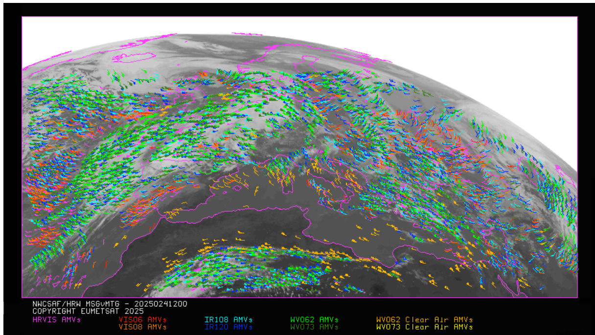
Figure 8: AMVs considering the satellite channel used for the AMV calculation, for the MSG series High Resolution Winds example defined in Figure 34 (24 January 2025, 12:00 UTC, Meteosat-10 satellite)
