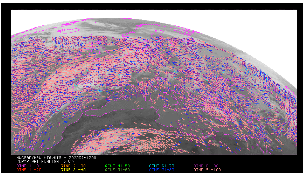
Figure 29: “Quality index without forecast” for the High Resolution Winds example defined in Figure 32 (24 January 2025 12:00 UTC, Meteosat-12 (MTG-I1) satellite). All values are formally possible for the “Quality index without forecast”, but because of its connection with the “Quality index with forecast”, only values of “Quality index without forecast” \geq 67\% are here really present.
