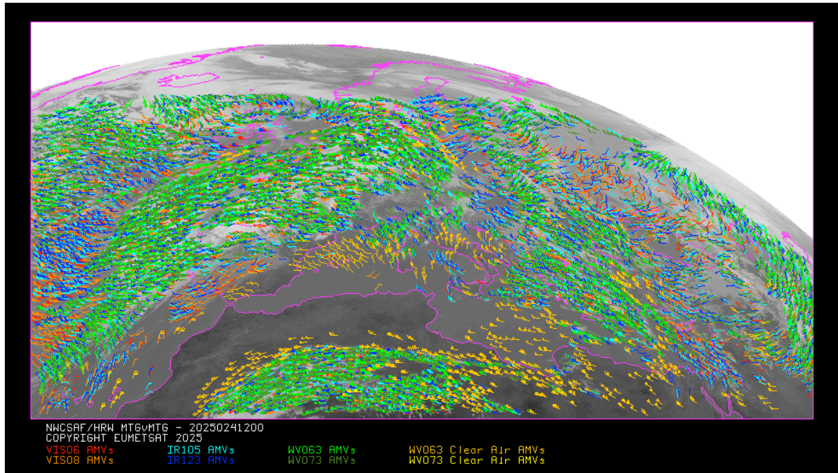
Figure 7: AMVs considering the satellite channel used for the AMV calculation, for the MTG-I series High Resolution Winds example defined in Figure 32 (24 January 2025, 12:00 UTC, Meteosat-12 (MTG-II) satellite)
