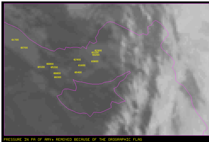
Figure 31: Pressure values in Pa for AMVs affected by orography (i.e. with “Orographic flag” values between 1 and 5) in a zoomed area around the island of Cyprus for an example case (Basic AMVs, Meteosat-9 satellite). Orographic effects are caused by the mountains in Cyprus and Turkey, reaching respectively 2000 m and more than 3000 m
