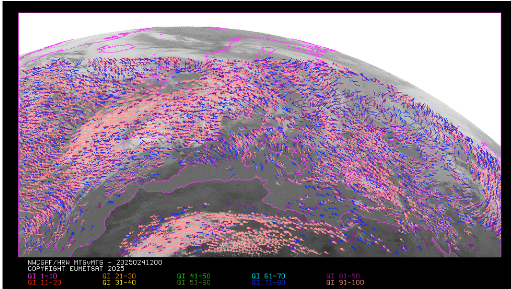
Figure 28: “Quality index with forecast” for the High Resolution Winds example defined in Figure 32 (24 January 2025 12:00 UTC, Meteosat-12 (MTG-I1) satellite). Only values of “Quality index with forecast” \geq 75\% are present because of the use of this parameter for the AMV filtering.
